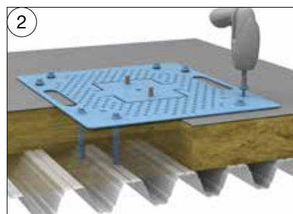
Position TATPLAT in the desired location and find the underlying crest in the plate. Push in the accompanying sleeves. 2 x in each corner, 8 in total. Fasten them with the accompanying screws.
