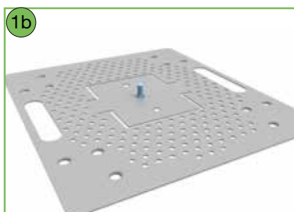
1b Install the carriage bolt in the TATPLAT from underneath, from bolt set 26 for bracket TSK or bolt set 27 for LLF150.
