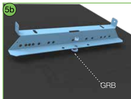
Mount TSK on TATPLAT. Use the accompanying rubber disc GRB under TSK and the accompanying nuts.
