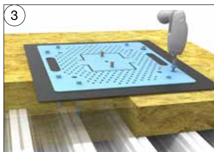
3 Position TATPLAT in the desired location and find the underlying crest in the plate. Push in the accompanying sleeves. 2 x in each corner, 8 in total. Fasten them with the accompanying screws.
