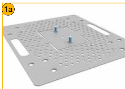
1a Install carriage bolts in TATPLAT from underneath. For UNIK.
