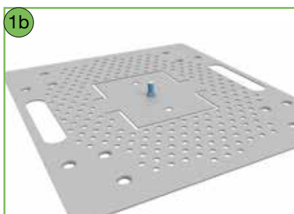
Install the carriage bolt/bolts in the TATPLAT from underneath. For bracket TSK or LLF150.
