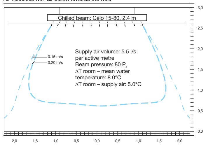
Air velocities with air blown towards the wall.
