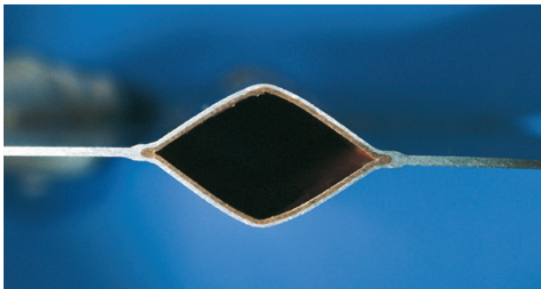
Picture 1. Cross-section of Lindab's unique strips. The rhomboid shape provides an efficient heat-transfer surface.
