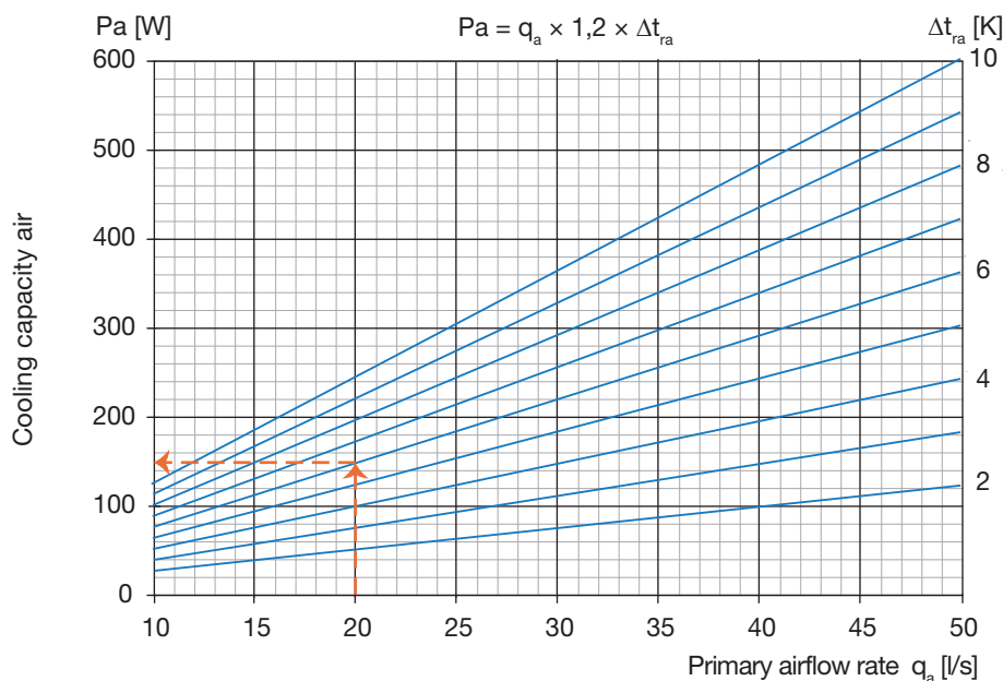
Diagram 1. Cooling capacity air Pa , as function of the primary airflow rate q_a . If the air supply is 20 l/s and the temperature difference of the room air and the supply air is \Delta t_{ra} = 6 \text{ K} , then the cooling capacity is 144 W.
