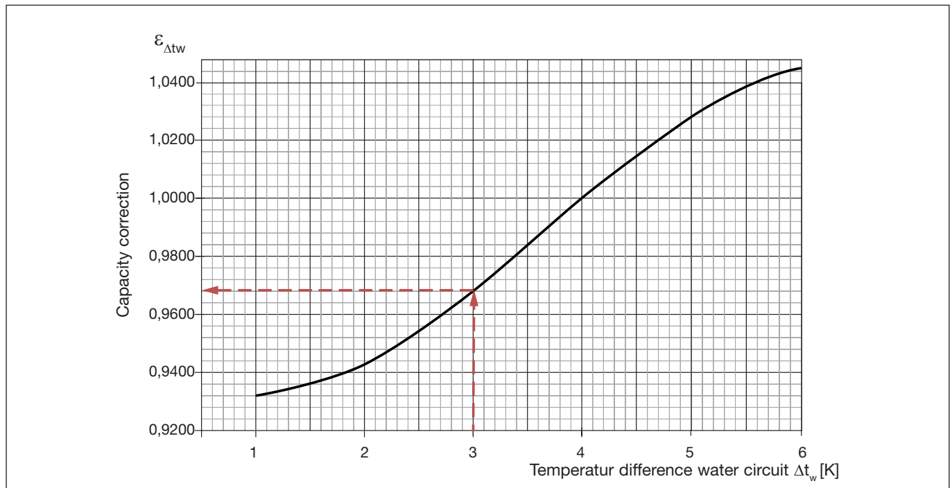
Diagram 5. Capacity correction \varepsilon_{\Delta t_w} as a function of \Delta t_w . Only applies for 2-pipe system, cooling or heating on Plexus 60.
