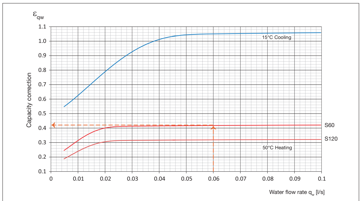
Diagram 8. Capacity correction for water flow \varepsilon_{qw} for both heating and cooling.
