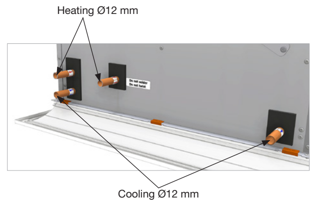
Picture 14. Water connections Plexus I-120. Cooling and heating.
