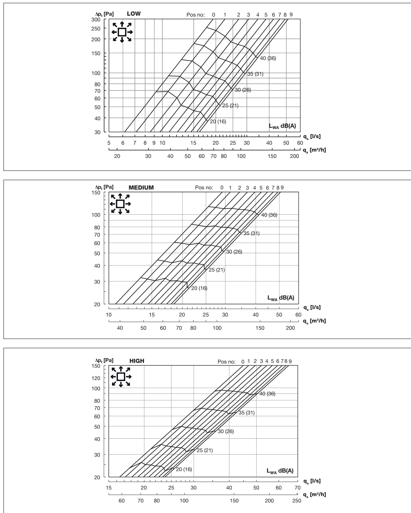
Diagram 12. Sound power level L_{WA} for Plexus 60 all models configuration Low/Medium/High.
