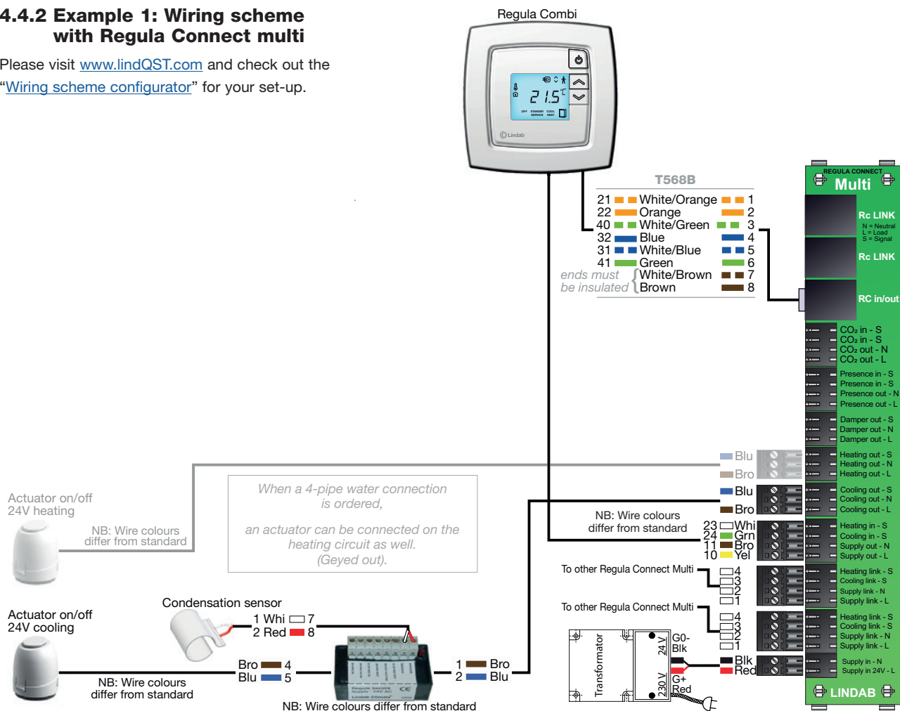
Example 1 Wiring scheme.
