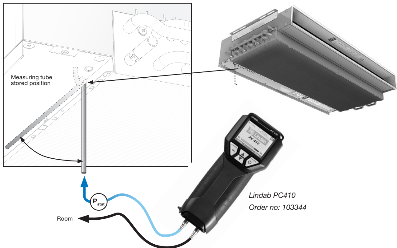
Measuring air flow.
