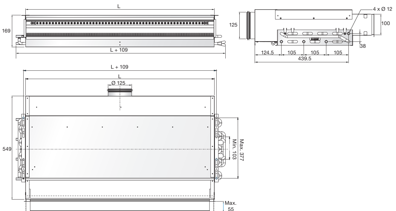
Dimension drawing.
