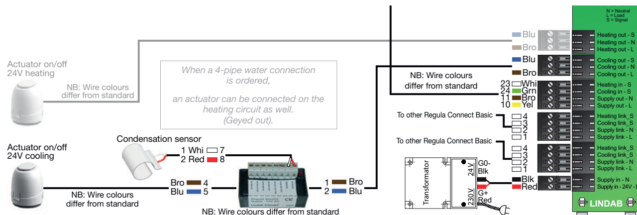
Example 2 Wiring scheme.
