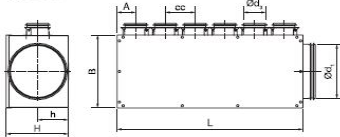
Type 6R
