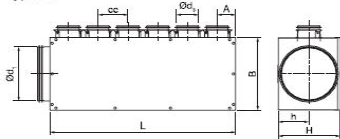
Type 6L
