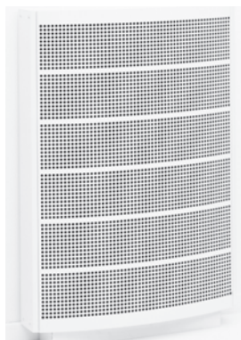
Ø7 deling kvadrat deling 10 mm feltperforeret friareal 38%
