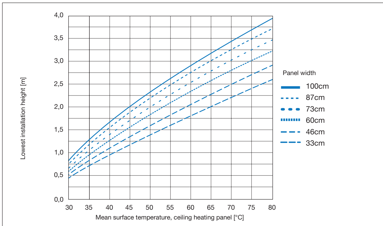
Lowest installation height for ceiling heaters with radiant temperature asymmetry of 5°C. Ceiling heater length 3.6 m.
