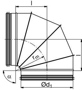
BKFU 90°, short, lockseamed bend
