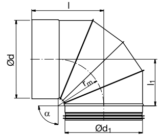
BKFMU 90°, short, segmented bend with female end
