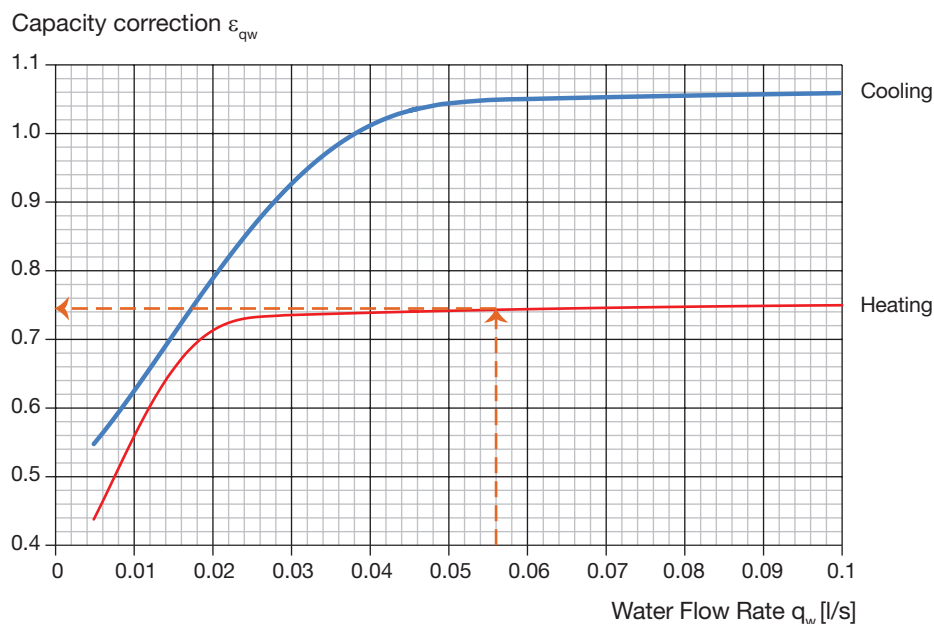
Diagram 3. Capacity correction \varepsilon_{qw} for water flow for both cooling and heating.
