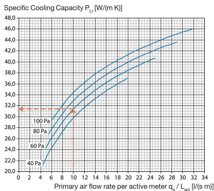
Diagram 2. Specific cooling capacity P_{Lt} as a function of primary air flow rate per active metre at nozzle pressures of 40, 60, 80 and 100 [Pa].
