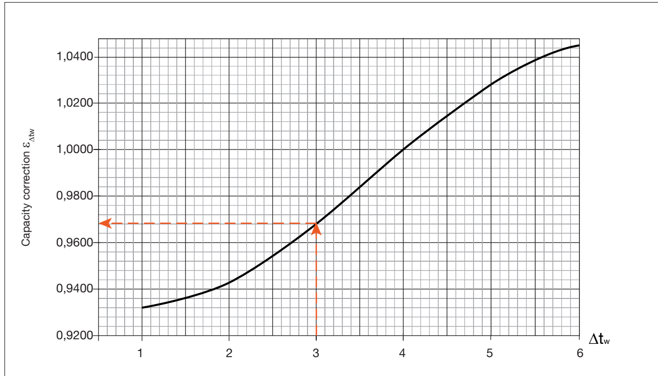
Diagram 4. Capacity correction \varepsilon_{\Delta t_w} as a function of \Delta t_w . Only applies for cooling.
