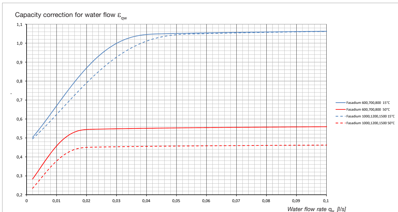
Diagram 5. Capacity correction \varepsilon_{q_w} for water flow for both cooling and heating.
