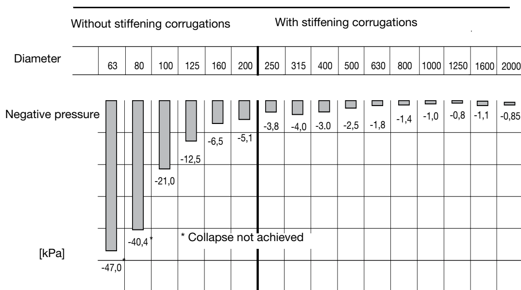
Collapsing pressure
