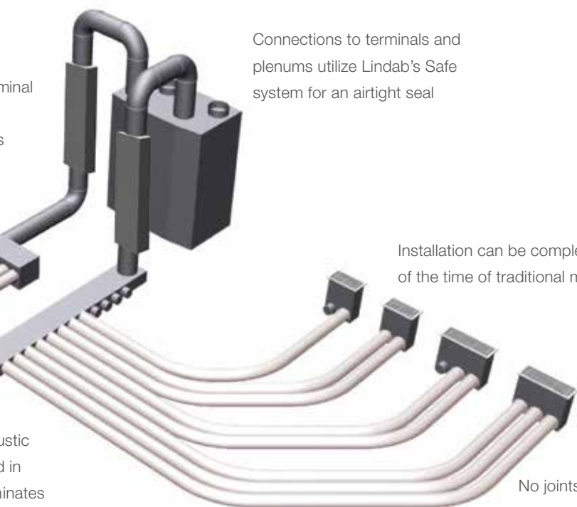
Bends are naturally gentle reducing turbulence, noise and pressure drop
