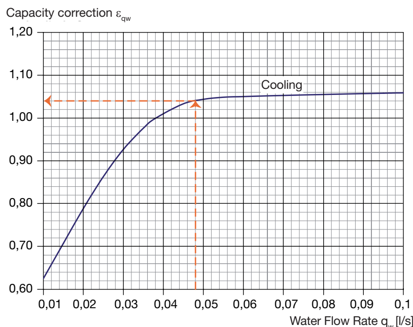
Diagram 3. Capacity correction \varepsilon_{qw} for water flow.
