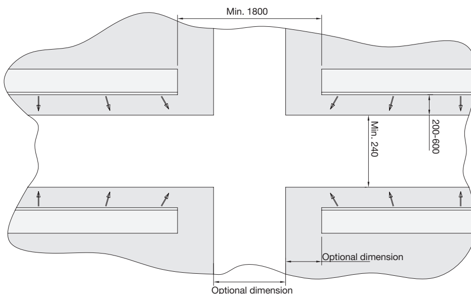
Figure 10. The picture shows four corners where suspended ceiling islands meet.
