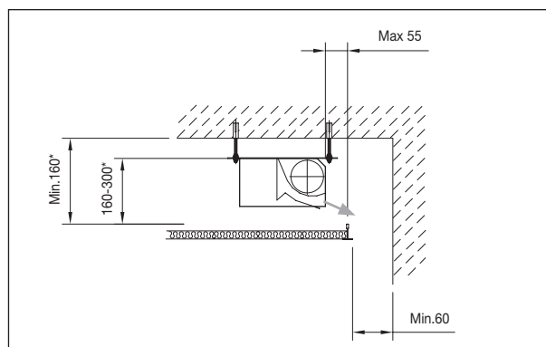
Figure 7. Dimensions for installation, outlet along the wall.
