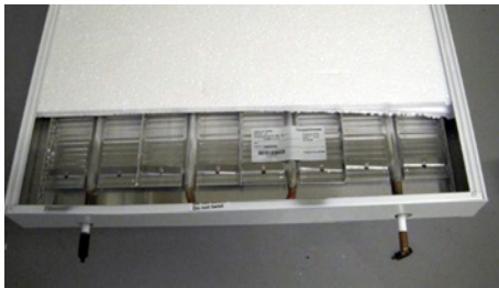
Atrium H Fig.2: Label location interior (Under insulation, above water connection).
