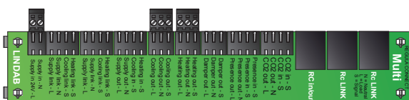
Picture 6. Weidmüller 1 x 2-pole-female (670290) and 2 x 3-pole-female (670291).
