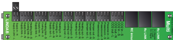
Picture 4. Weidmüller 2-pole-female (670290).
