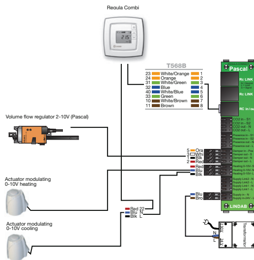
Picture 9.B. NOTE! When a heating actuator added to the system the the 2-pole weidmüller plug is replaced with a 3-pole plug which now is shared by the two actuators. The cooling actuator red wire is still connected to the Regula Combi plinth 22.
