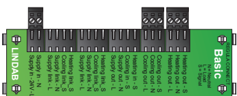
Picture 3. Weidmüller 1 x 2-pole-female (670290) and 2 x 3-pole-female (670291).
