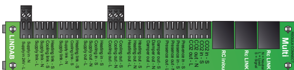
Picture 5. Weidmüller 1 x 2-pole-female (670290) and 1 x 3-pole-female (670291).
