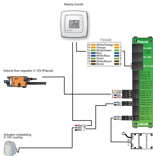
Picture 8.B. NOTE! The Cooling actuator red wire is connected to the Regula Combi plinth 22 and the 2 other wires are connected to the Pascal card via a 2 Weidmüller 2-pole plug.
