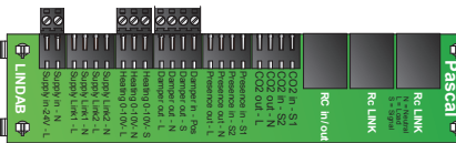
Picture 9. 1 x Weidmüller 2-pole female ( for power supply, always included), 1 x 3-pole female+ 1 x 4 pole male. See picture 9.B for simplified Wiring scheme configurator shot.
