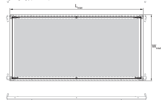
Figure 13. Inlet faceplate -3S dimensions.
