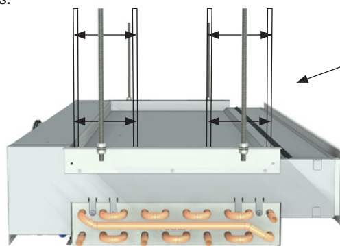
Picture 13. Munio-I suspension. Different types of hangers are available as accessory.
