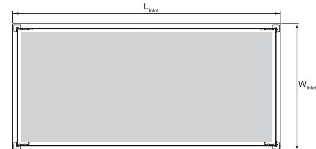
Figure 14. Inlet faceplate -01/-21 dimensions.
