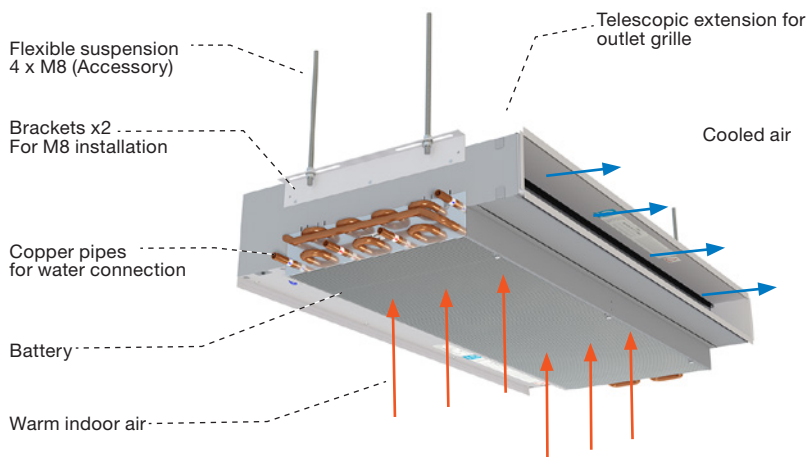
Picture 2a/b. Standard Munio-I-1000 (without inlet faceplate) parts and function principle.
