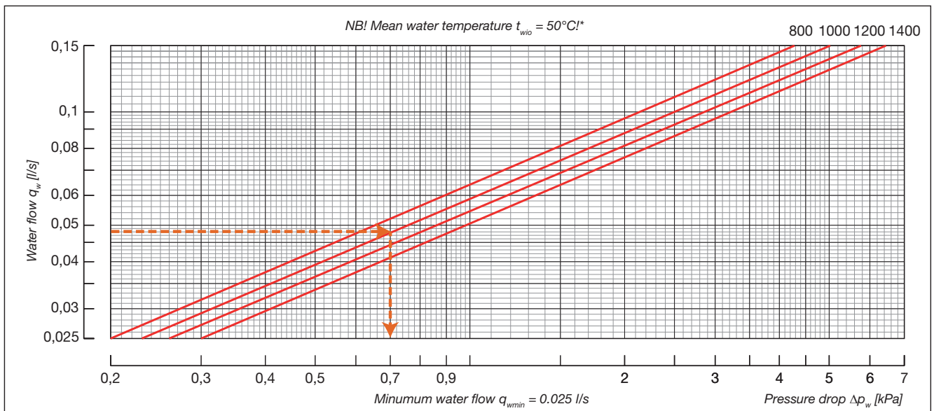
Diagram 5.b: Pressure drop in water circuit, heating.
