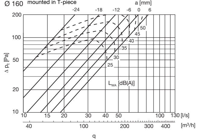
Ø 160 mounted in T-piece
