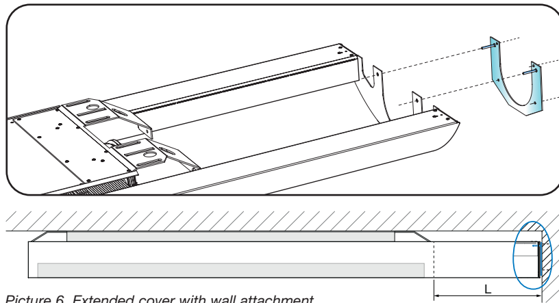
Picture 6. Extended cover with wall attachment.
