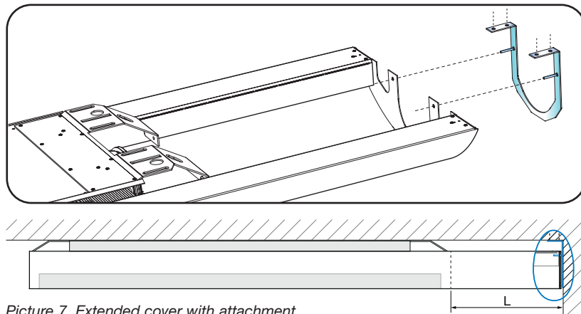
Picture 7. Extended cover with attachment installed on ceiling.
