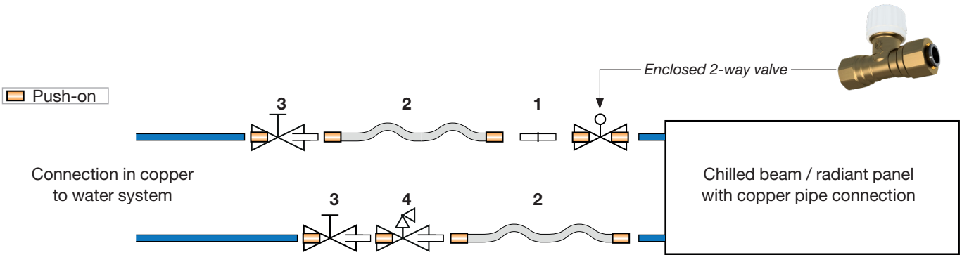
Picture 4. Connection to a 2-pipe unit - with enclosed 2-way valve).
