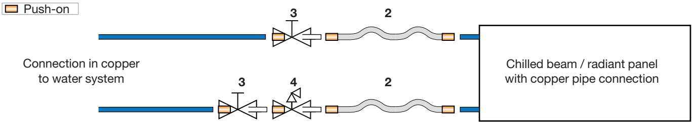
Picture 3. Connection to a 2-pipe unit - directly (without enclosed 2-way valve).
