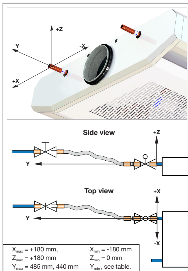
Picture 15. Max. distance between beam/panels and water system.
