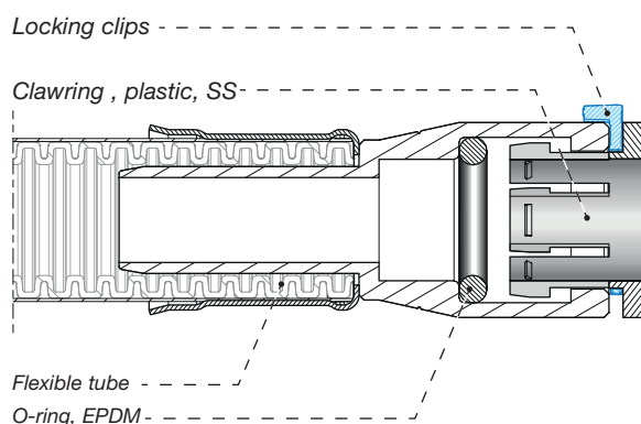
Picture 6. Section view of Lindab push fittings.
