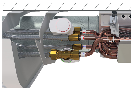
Picture 2. 4-pipe water connection with 2x Linflow-S valves and flexible hoses (Plafond XD).
