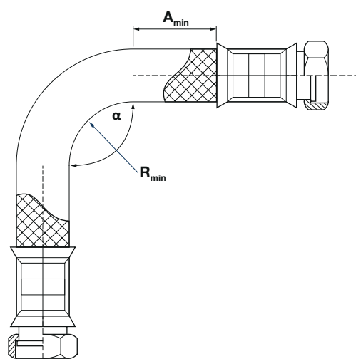
Picture 9. Flexible hoses, minimum bend radius.
