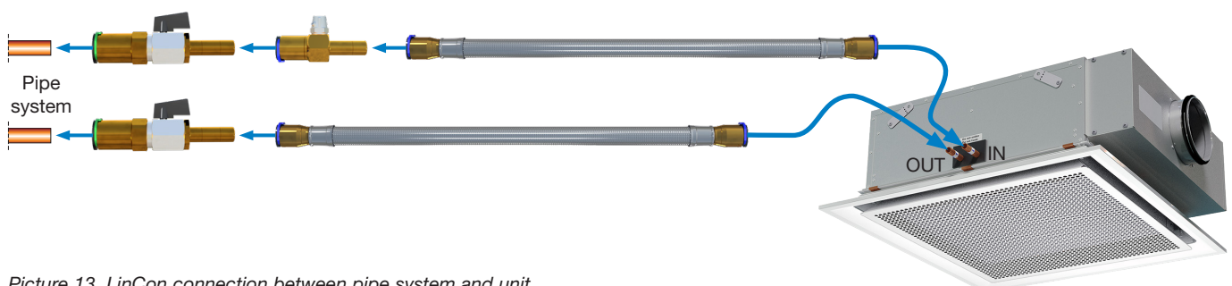
Picture 13. LinCon connection between pipe system and unit
