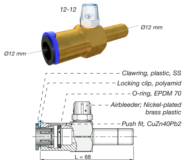
Picture 12. Section view of Air vent - Connector with airbleeder.
