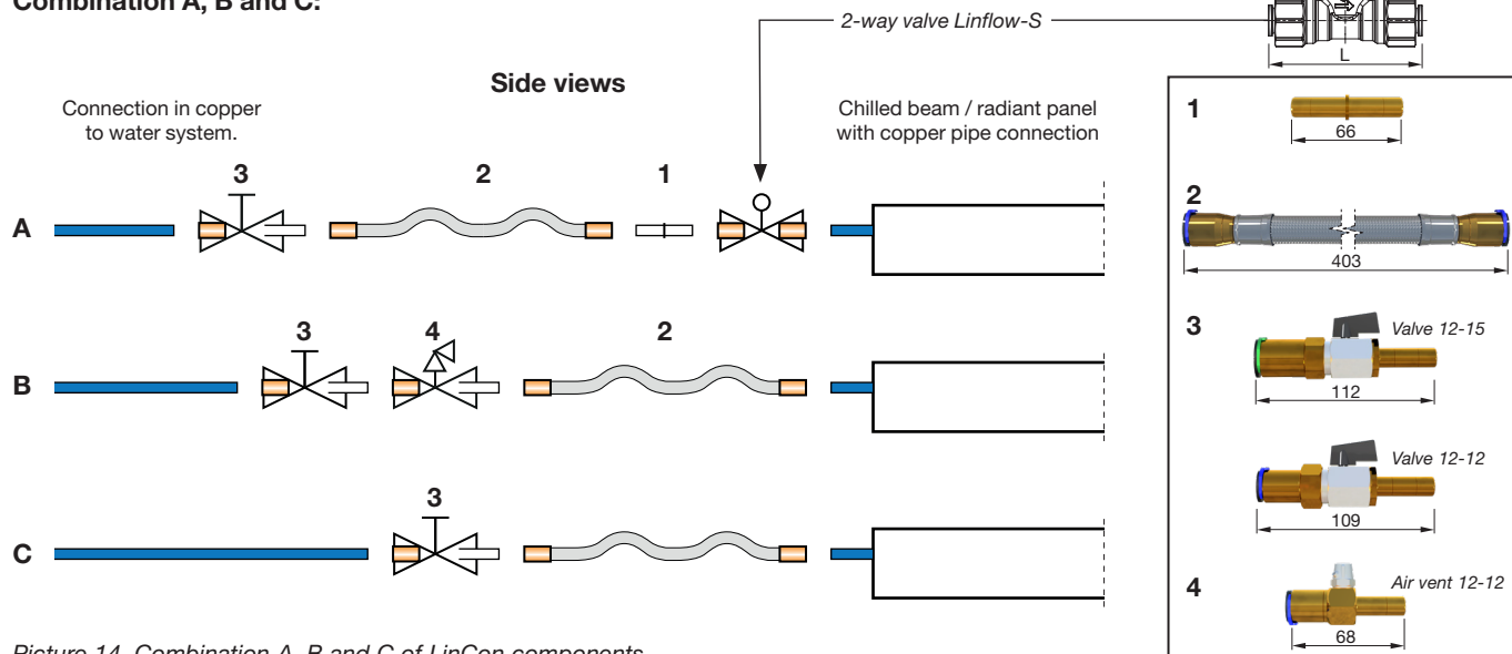
Picture 14. Combination A, B and C of LinCon components.
