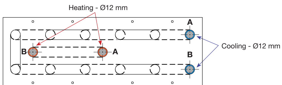
Figure 4 Fasadium: 1000, 1200, 1500
