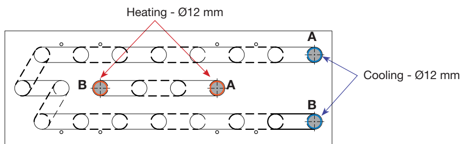
Figure 3. Fasadium: 600, 700, 800
