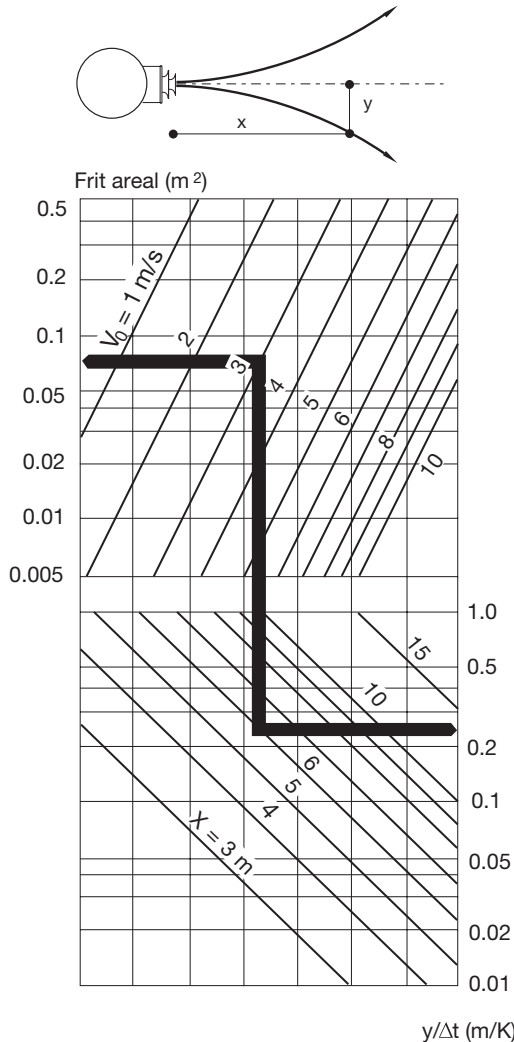
Fig. 14, Planning mixed ventilation.
