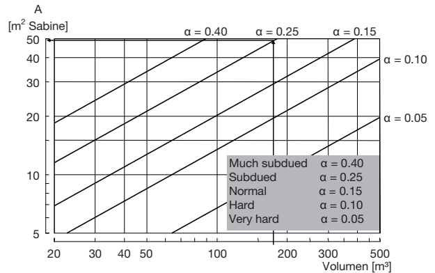
Fig. 26, Direction factor for different placements of sound sources and the relationship between the room volume and equated sound-absorption area.
