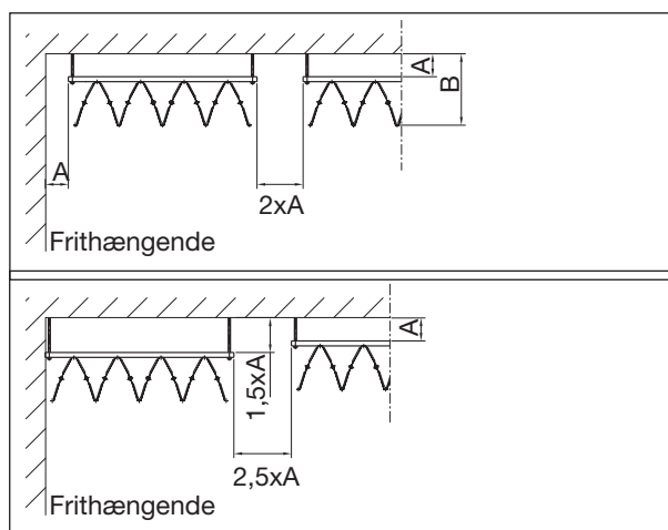
Figure 2-4. Installation dimensions for Carat.
