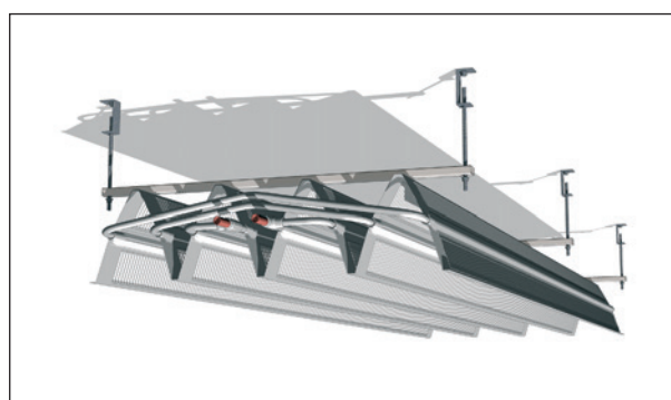
Picture 10. Installation of Carat with threaded rods.
