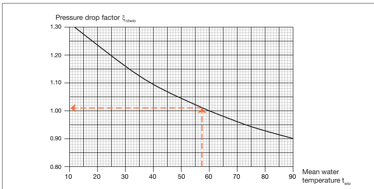
Diagram 5. Temperature adjusted pressure drop factor.
