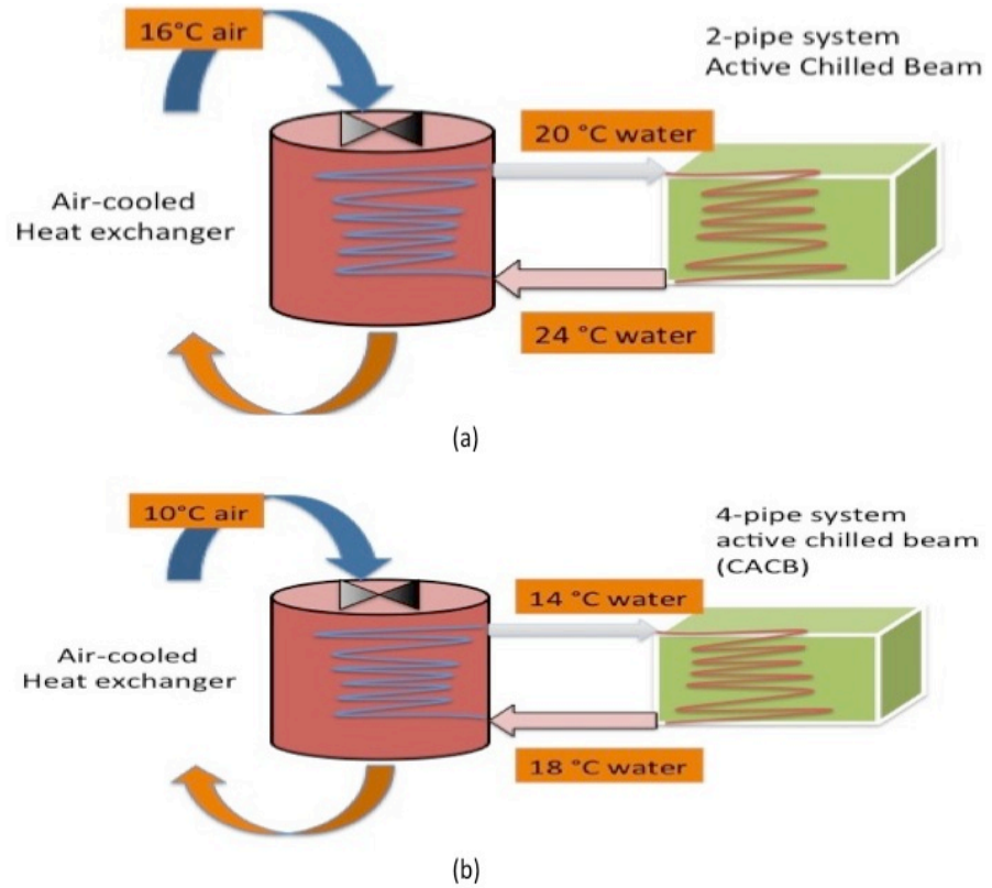
Figure 11(a) free cooling scenario 1 for the Two-Pipe System (b) free cooling scenario 1 for the CACB system.
