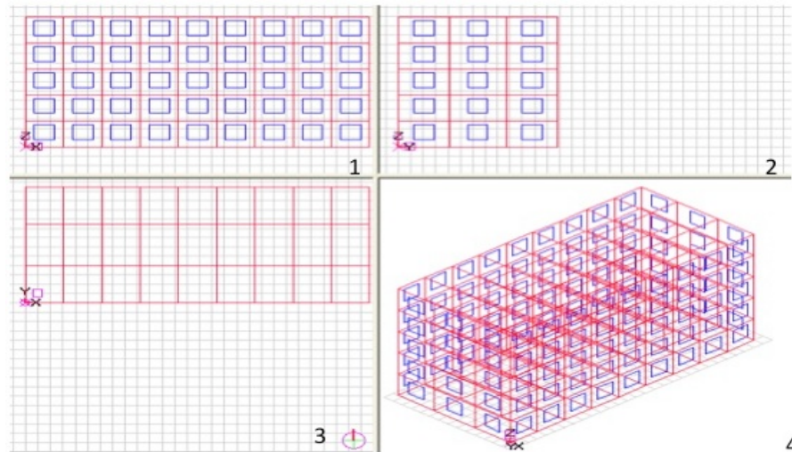
Figure 6 Building geometry in BSim; 1: South view, 2: East view, 3: Top view, 4: 3-D view.
