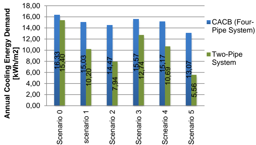
Figure 16 Annual cooling energy demand; Two-Pipe System vs. CACB in different scenarios.
