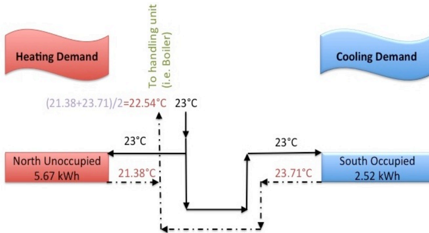
Figure 18 Schematic view of simulated energy transfer on 16th February 12:00-13:00.
