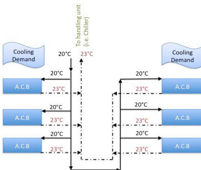
Figure 4 Two-Pipe System Schematic view when there is only cooling demand. [18]
