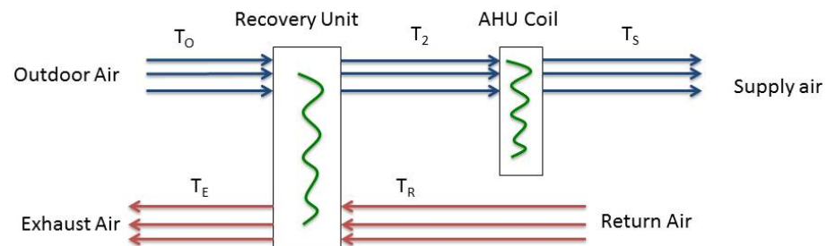
Figure 8 Ventilation system.
