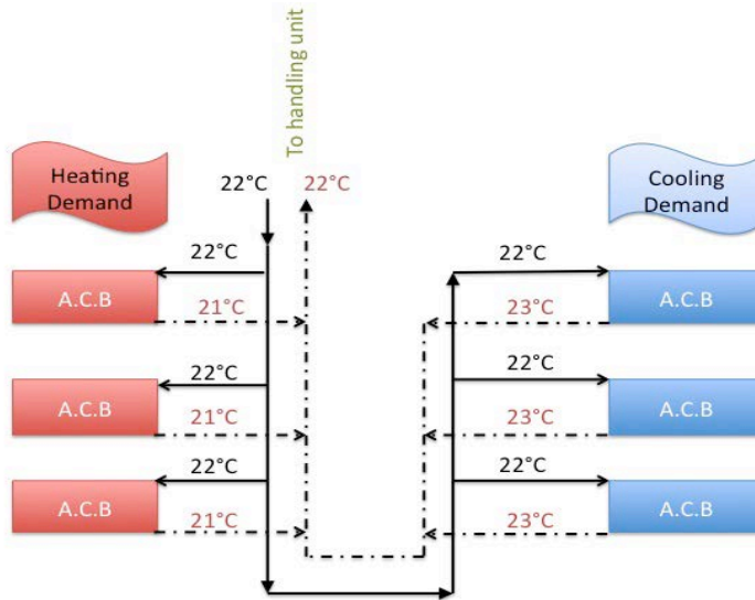
Figure 2 Two-Pipe System Schematic view when there are equal cooling demand and heating demands simultaneously. [18]
