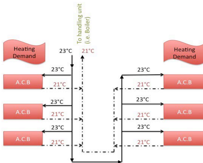
Figure 3 Two-Pipe System Schematic view when there is only heating demand. [18]
