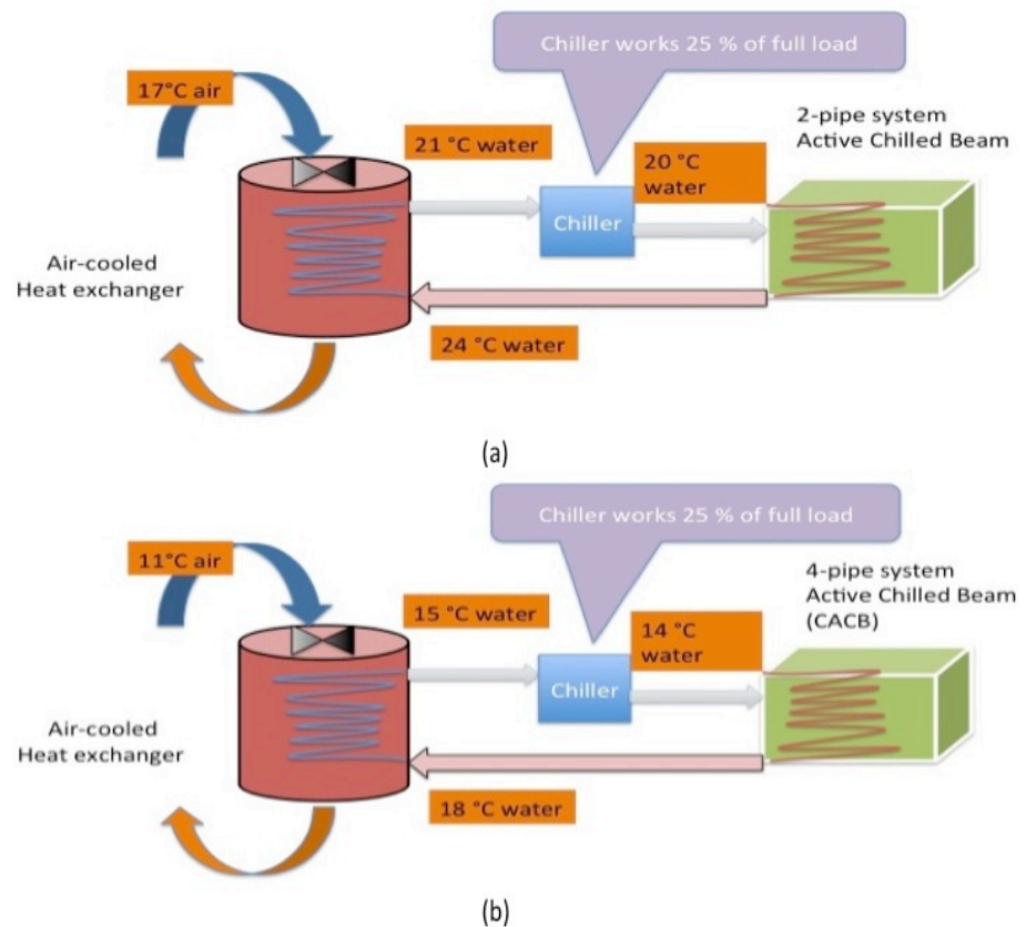
Figure 12(a) 75% free cooling in scenario 4 for the Two-Pipe System (b) 75% free cooling scenario 4 for the CACB.
