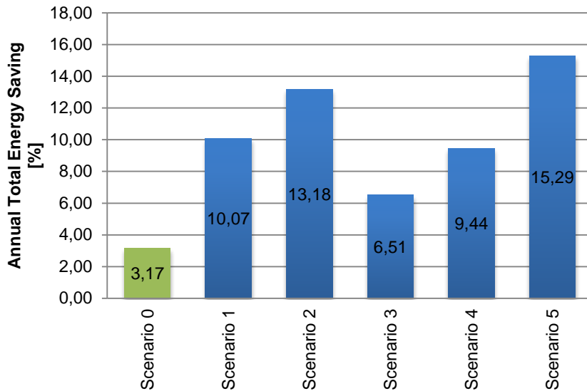
Figure 20 Percentage of energy saved by using the Two-Pipe System vs. the CACB.
