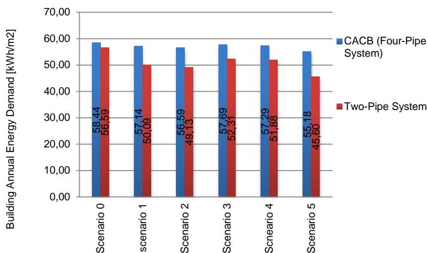
Figure 14 total energy demand in different scenarios, Two-Pipe System vs. CACB.
