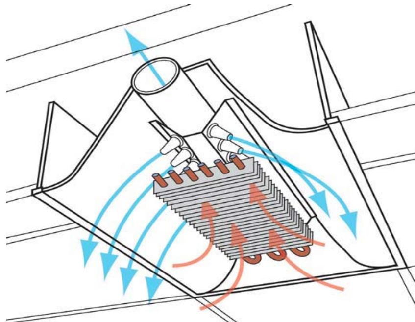
Figure 1 Active chilled beam air streams: Blue streams are primary air and red streams are induced air to the coil [2].
