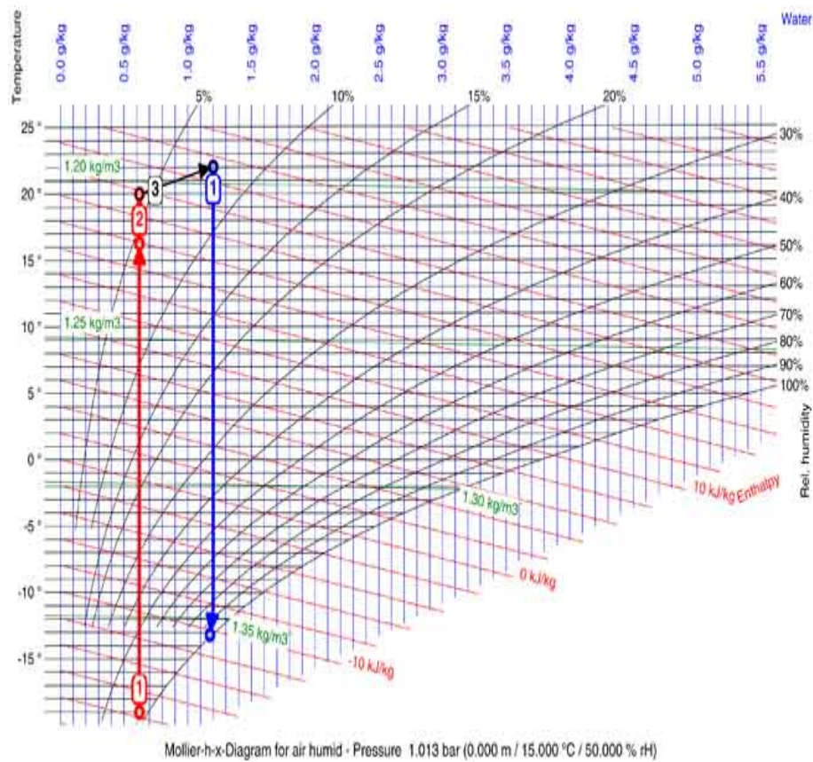
Figure 22 Mollier diagram.
