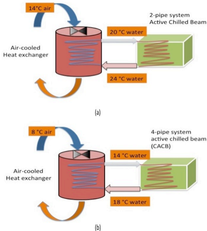
Figure 10(a) free cooling scenario 3 for the Two-Pipe System (b) free cooling scenario 3 for the CACB system.
