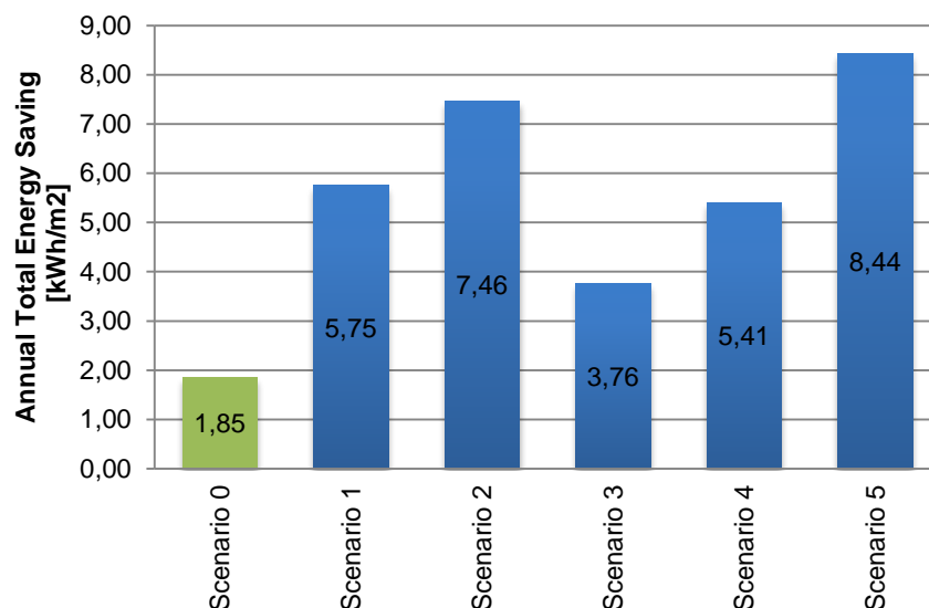
Figure 19 Annual total energy saving through energy transfer in Two-Pipe System vs. CACB.
