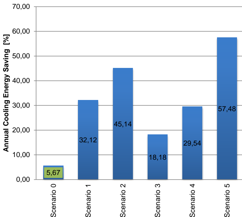
Figure 21 Annual cooling energy saving percentage for Two-Pipe System vs. the CACB.
