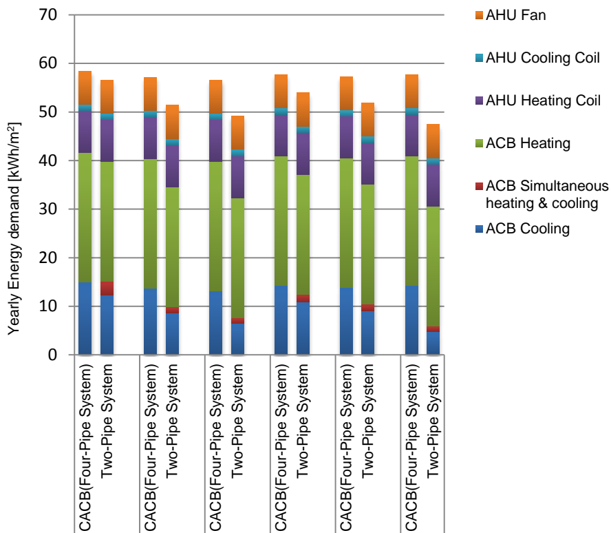
Figure 15 Yearly Energy Demand for the Two-Pipe System vs. the CACB.
