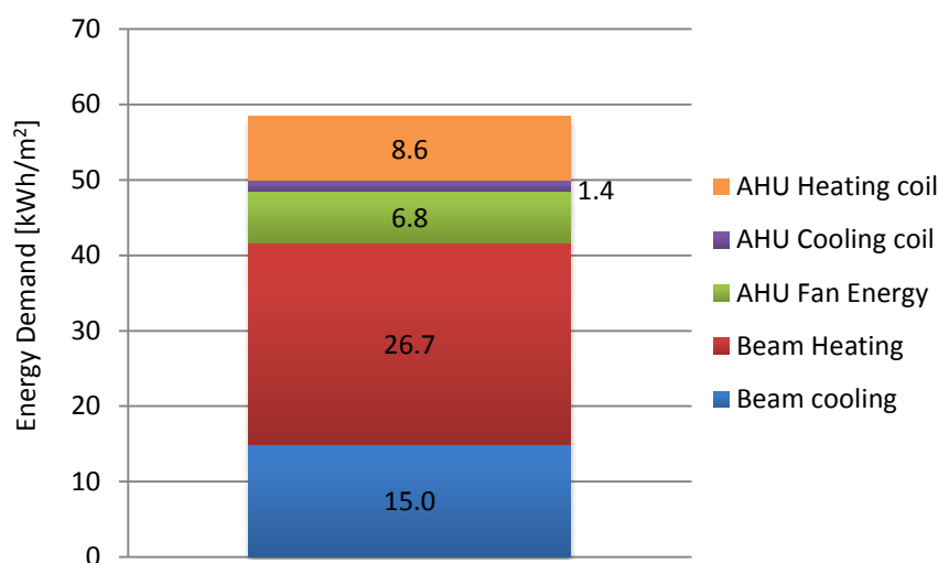
Figure 13 Annual energy demand in building model from BSim software.
