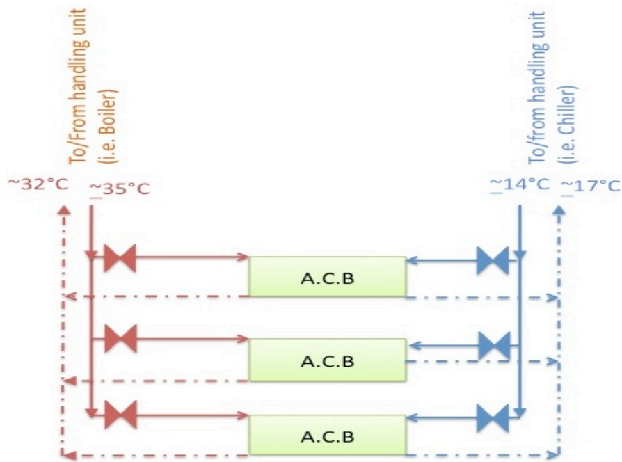
Figure 5 Schematic view of the CACB beam application. [18]
