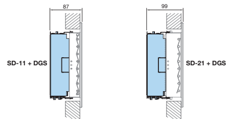
Grille with 1 row of blades. Grille with 2 rows of blades.
