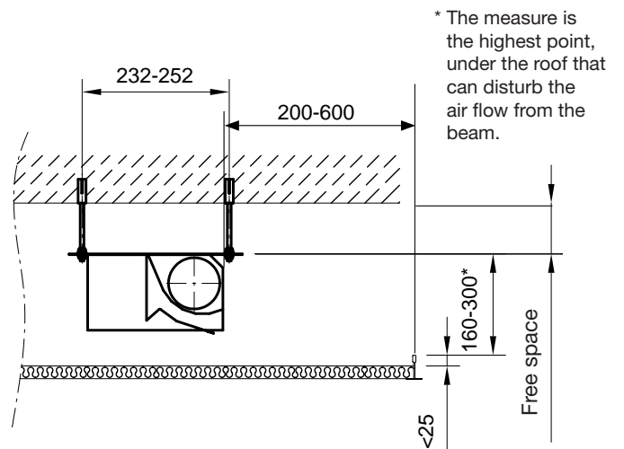
Figure 3. Island mounting
