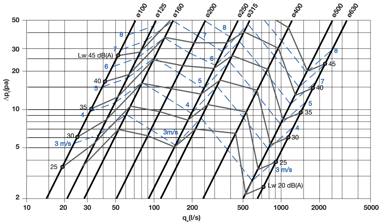
Model 3 and 4 Pressure loss and sound generation for 100 and 1250 mm long attenuators ( \phi d_1 400 - 630 \rightarrow (l) = 1250 mm)
