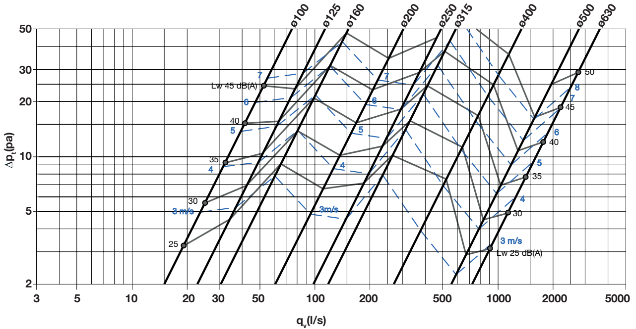
Model 3 and 4 Pressure loss and sound generation for 600 mm long attenuators
