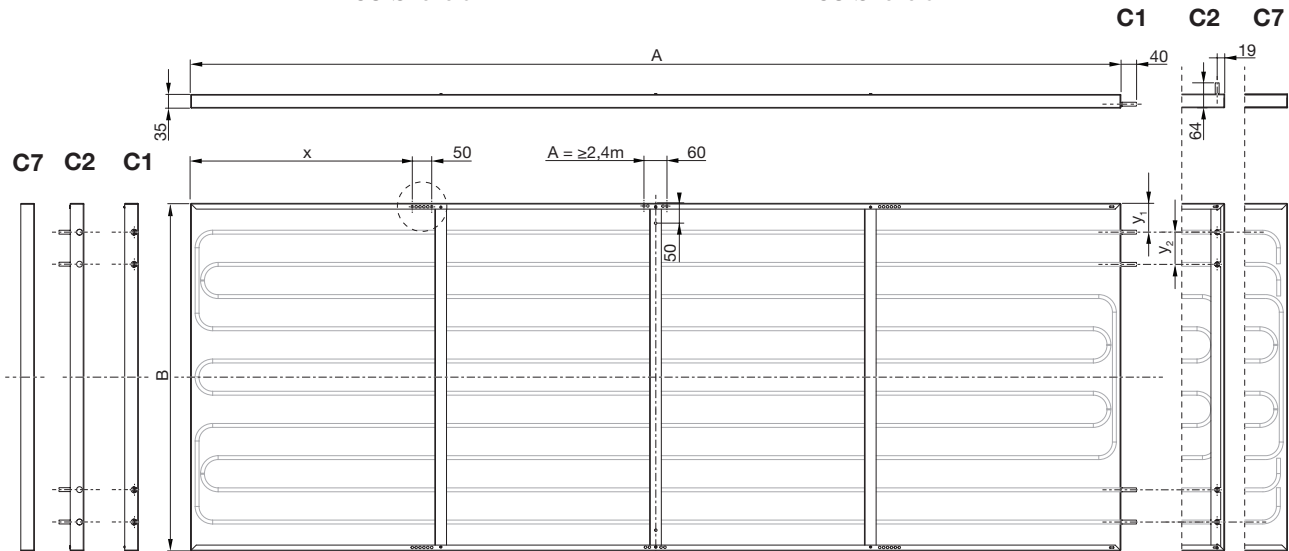
Dimensions of heating and cooling panel
