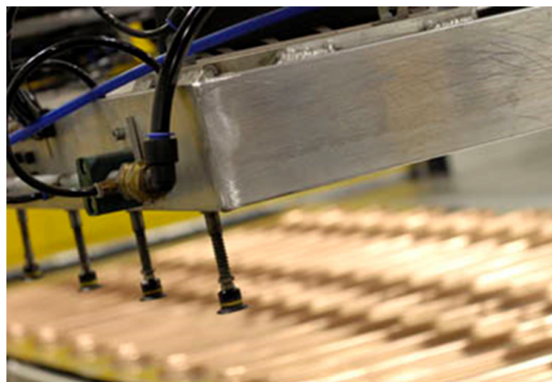
Picture 1: Atrium Plana unique manufacturing process.
