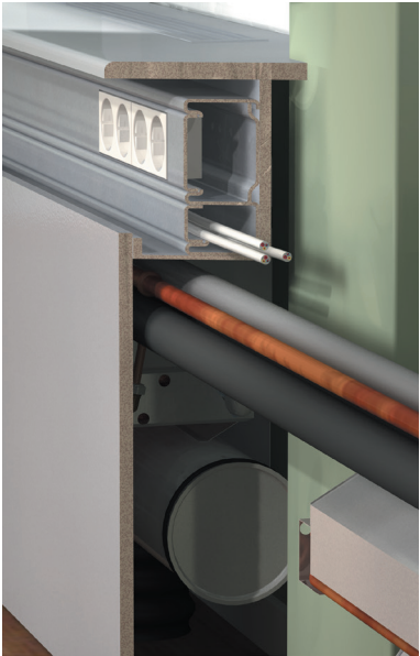
Picture 7. Casing with fixed worktop and visible electrical cable duct.
