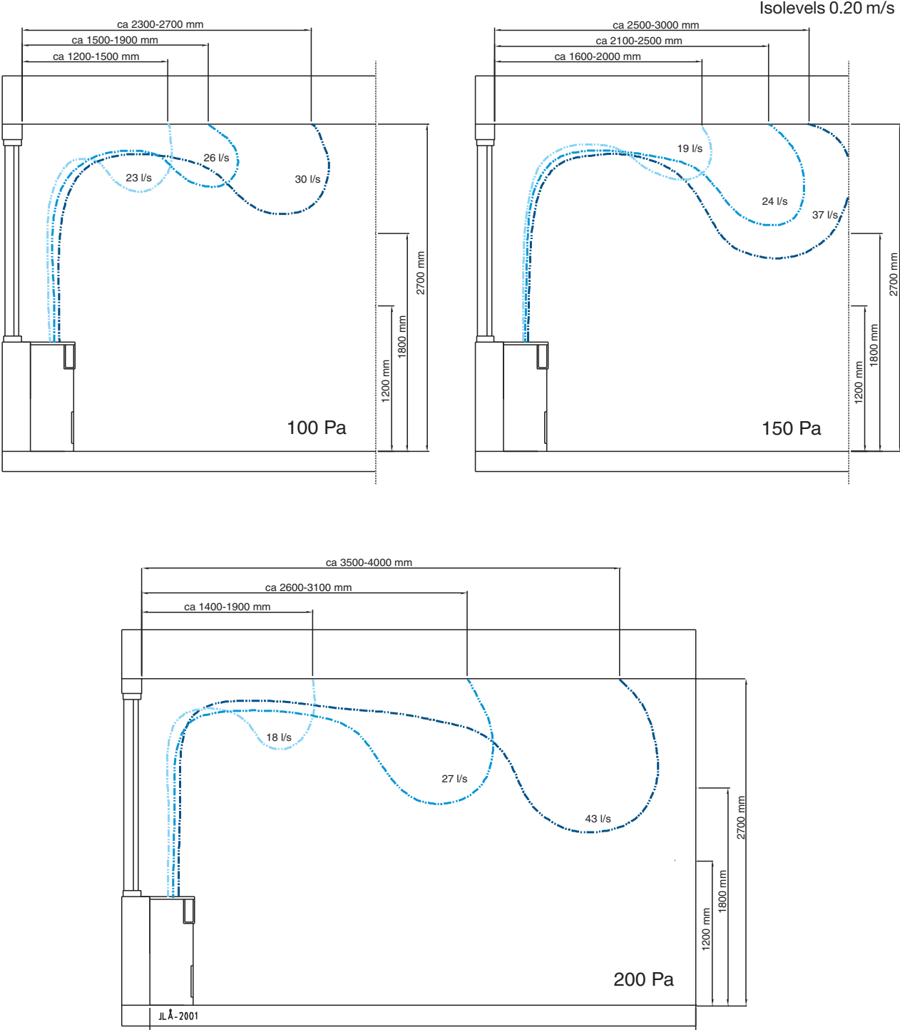
Figure 6. Fasadium – 1200 distribution diagrams, different air and flow settings.
