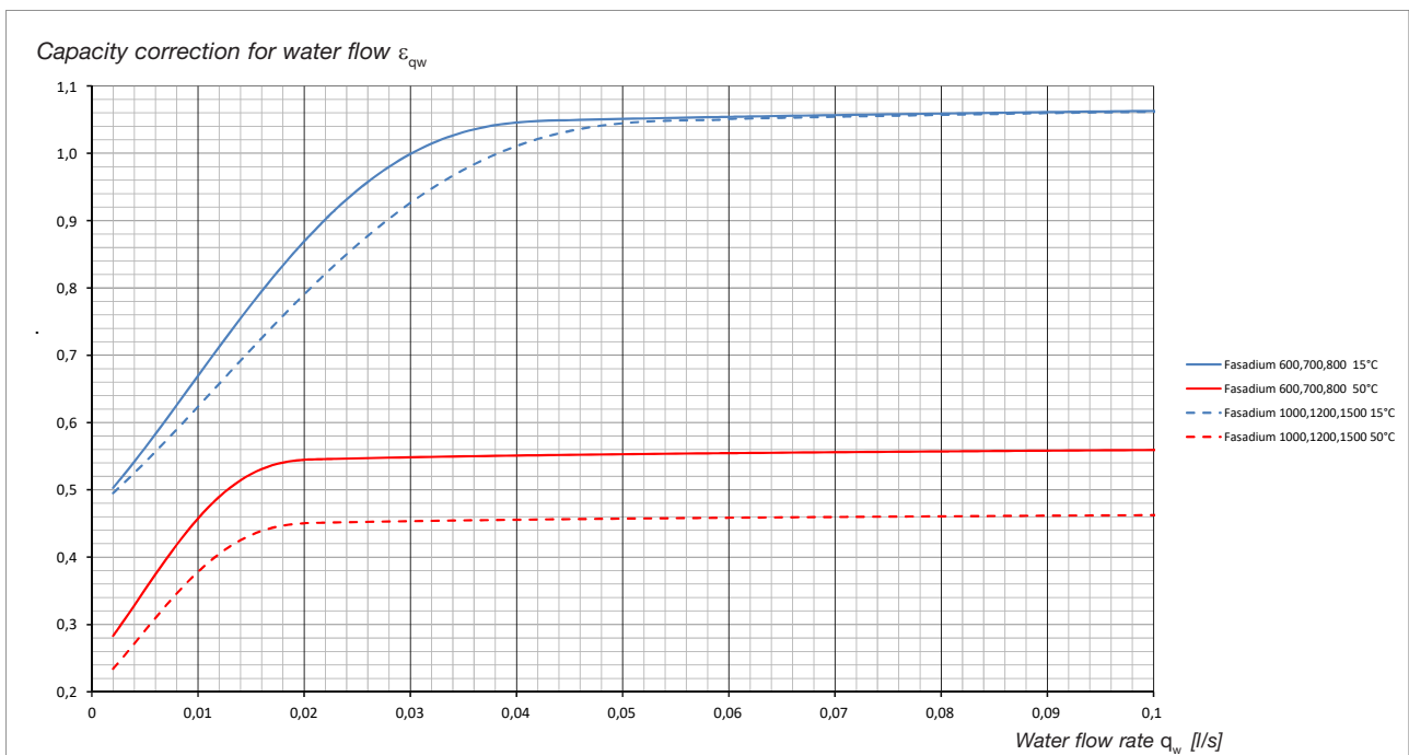
Diagram 5. Capacity correction \epsilon_{q_w} for water flow for both cooling and heating.
