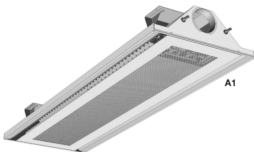
Figure 4. Examples of the most common Premum supply air A and B variants. Go to next page to see overview of various water pipe connections.
