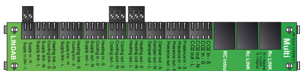
Picture 6. Weidmüller 1 x 2-pole-female (670290) and 2 x 3-pole-female (670291).
