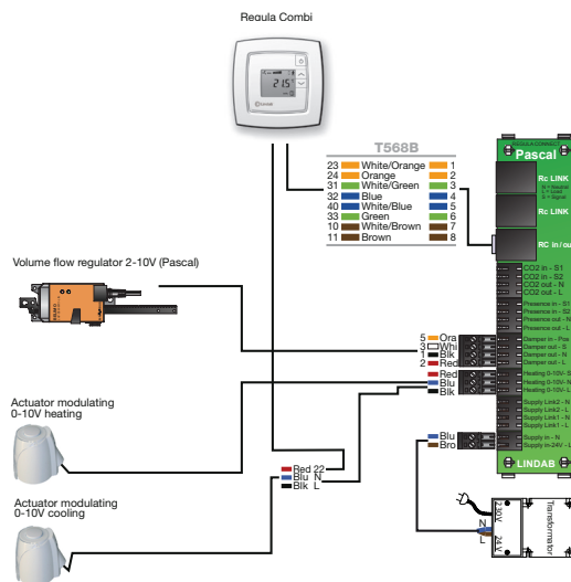
Picture 9.B NOTE! When a heating actuator added to the system the the 2-pole weidmüller plug is replaced with a 3-pole plug which now is shared by the two actuators. The cooling actuator red wire is still connected to the Regula Combi plinth 22.
